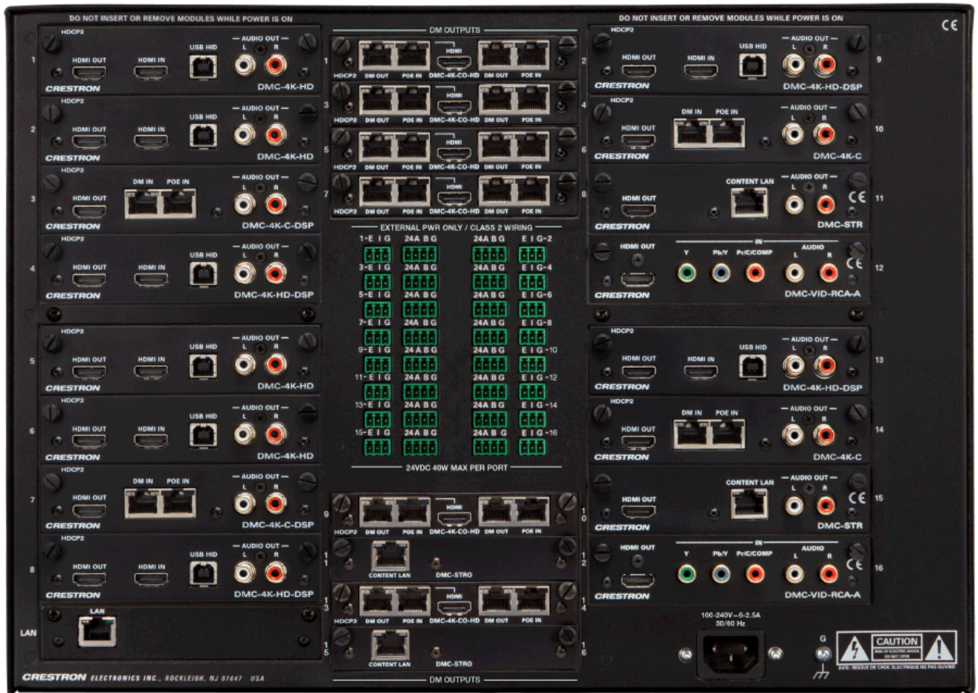
DM-MD16X16-RPS – Rear view with I/O cards installed
