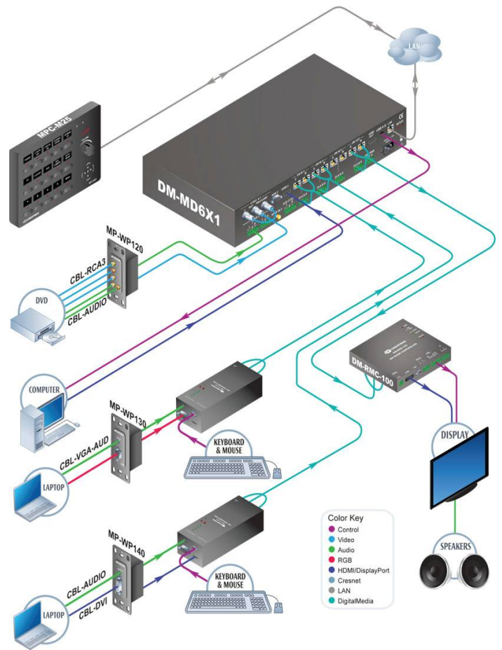
DigitalMedia: DM-MD-6X1 HDMI Switcher Application
