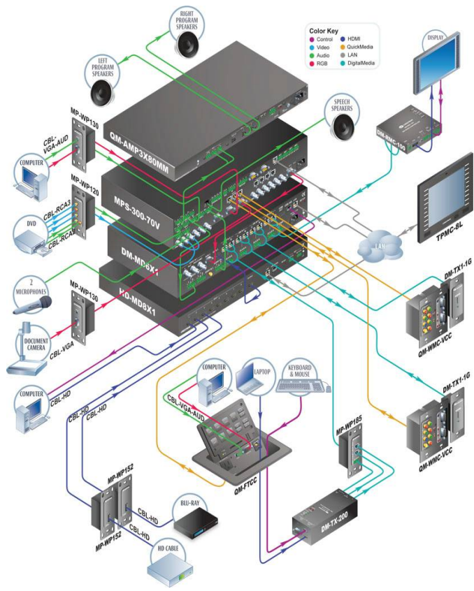
DigitalMedia: Commercial Conference Room with MPS, QM and DM Components
