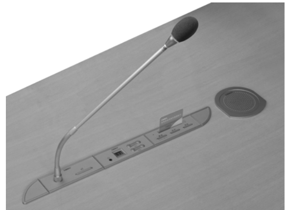
Combination of N-style units (flush-mounting)
