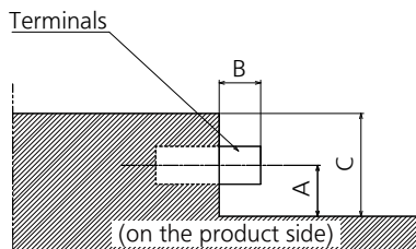
Sectional view of terminal b USB/AUDIO OUT/AUDIO IN/PC IN/DVI-D IN/HDMI 1/HDMI 2
