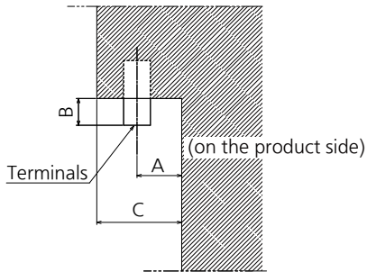
Sectional view of terminal a SERIAL IN/IR IN
