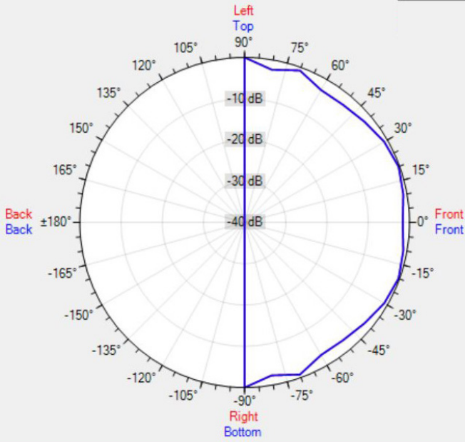
Data Shown: CMAR8 (Apart Audio) Display Parameters: Frequency: 1000Hz (1/24th Octave)
