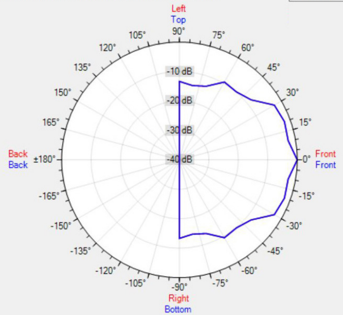
Data Shown: CMAR8 (Apart Audio) Display Parameters: Frequency: 8000Hz (1/24th Octave)
