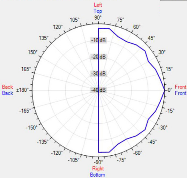
Data Shown: CMAR8 (Apart Audio) Display Parameters: Frequency: 4000Hz (1/24th Octave)
