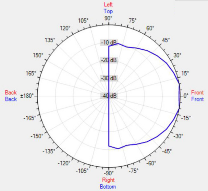
Data Shown: CMAR8 (Apart Audio) Display Parameters: Frequency: 2000Hz (1/24th Octave)
